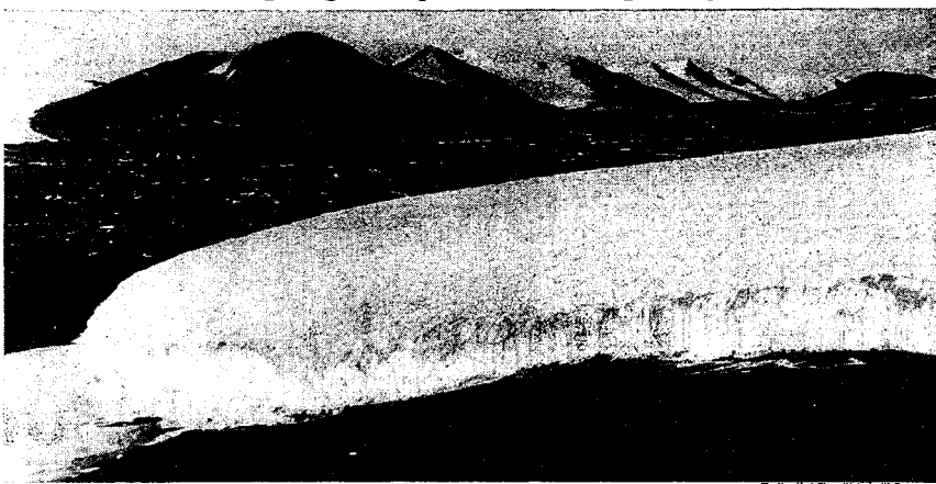
Tongue of Antarctic ice sheet that invades valleys west of McMurdo Sound. If scientists wish to see how last ice age looked, they visit the continent. The New York Times/Matczak W. Brown
