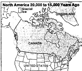
North America 20,000 to 15,000 Years Ago The New York Times/May 21, 1975 Shortly after its last major advance, the ice sheet covered almost all of Canada and much of the northern United States. Some scientists now believe, on the basis of recent findings, that ice resting on the sea floor extended far off the shore. The map is adapted from "The Earth and Its History" by R.F. Flint.
