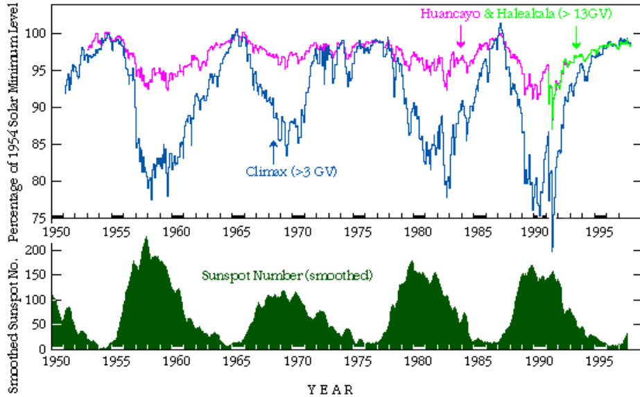
Figure 8: Variation with time of sunspot number and cosmic ray flux, as measured by ground-based neutron counters. The neutron data are from the Univ. Chicago Neutron Monitor Stations at Climax, Colorado (3400 m elevation; 3 GeV primary charged particle cutoff), Huancayo, Peru (3400 m; 13 GeV cutoff) and Haleakala, Hawaii (3030 m; 13 GeV cutoff). The stronger modulation of the cosmic ray flux at higher latitudes (Climax) is due to the lower primary cutoff energy.
