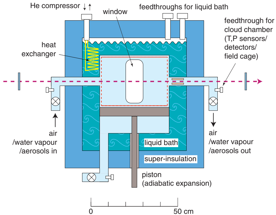
Figure 17: Schematic diagram of the CLOUD chamber.
